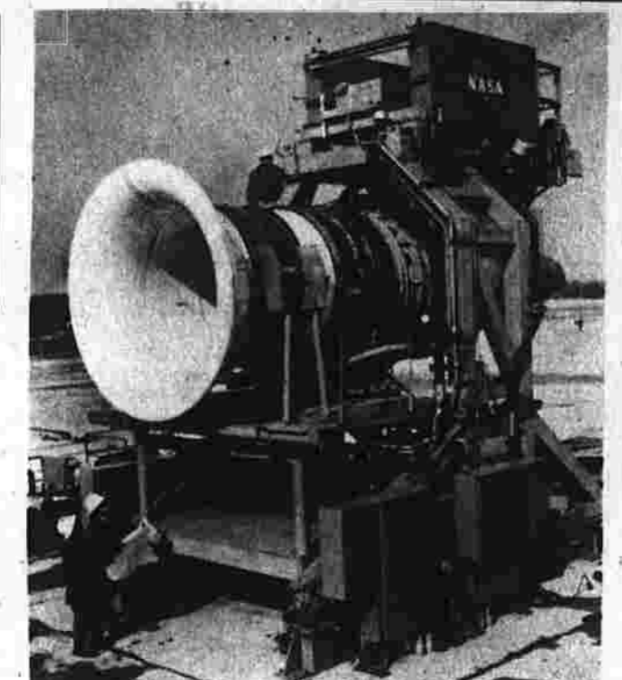
NOT POWER but noise, or lack of it, is the point of a design new jet engine under test at NASA's Lewis Research Center in Cleveland. The "Quiet Engine" is planned to cut noise levels at jet airports.
